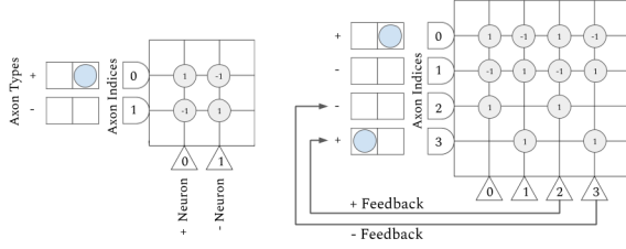
Fig. 7. RANC allows signed VMM without feedback (left) while the equivalent operation on TrueNorth requires feedback (right).
